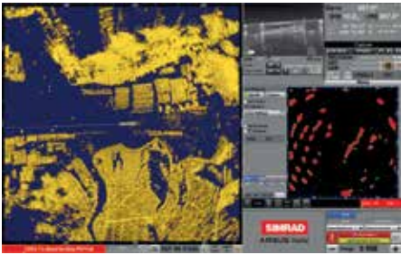
Argus S-Band - standard PPI screen showing dual range
